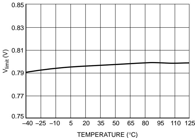
Figure 33. Maximum Internal Current Set-point, V_{limit}
