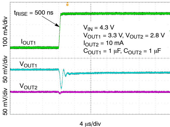
Figure 46. Load Transient Response – 3.3 V – Rising Edge, I_{OUT1} = 100 μA to 300 mA
