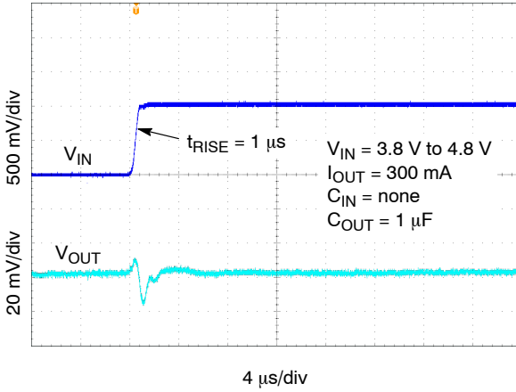
Figure 36. Line Transient Response– Rising Edge, V_{OUT} = 3.3 V, I_{OUT} = 300 mA
