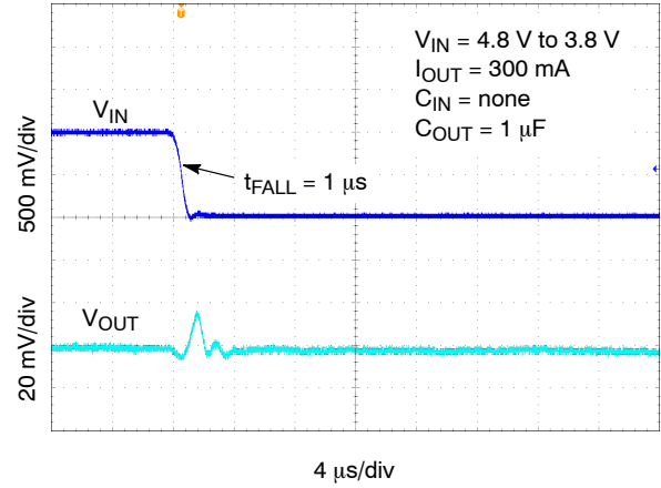
Figure 37. Line Transient Response– Falling Edge, V_{OUT} = 3.3 V, I_{OUT} = 300 mA
