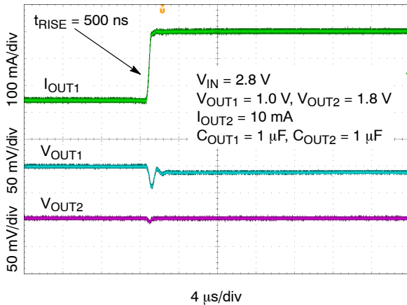
Figure 44. Load Transient Response – 1.0 V – Rising Edge, I_{OUT1} = 50 mA to 300 mA
