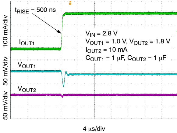
Figure 42. Load Transient Response – 1.0 V – Rising Edge, I_{OUT1} = 1 mA to 300 mA
