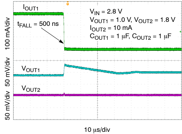
Figure 43. Load Transient Response – 1.0 V – Falling Edge, I_{OUT1} = 300 mA to 1 mA
