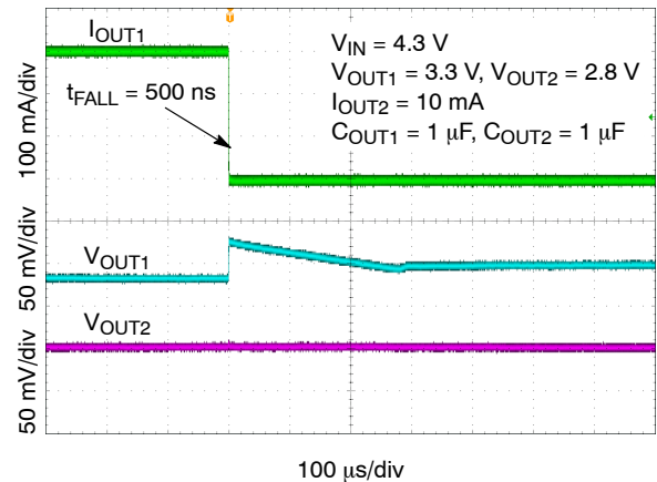
Figure 47. Load Transient Response – 3.3 V – Falling Edge, I_{OUT1} = 300 mA to 100 μA
