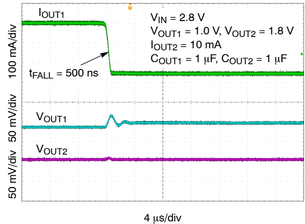
Figure 45. Load Transient Response – 1.0 V – Falling Edge, I_{OUT1} = 300 mA to 50 mA
