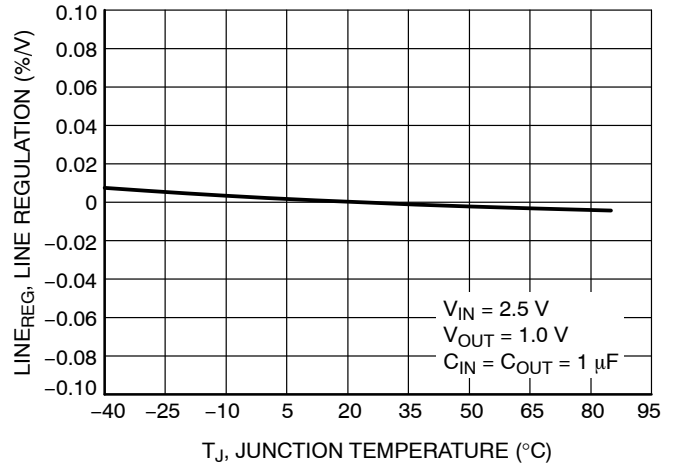
Figure 10. Line Regulation vs. Temperature – V_{OUT} = 1.0 V
