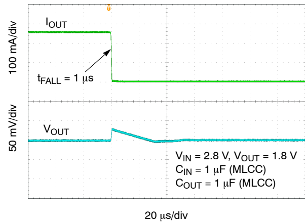
Figure 45. Load Transient Response – 250 mA to 1 mA – V_{OUT} = 1.8 \text{ V}
