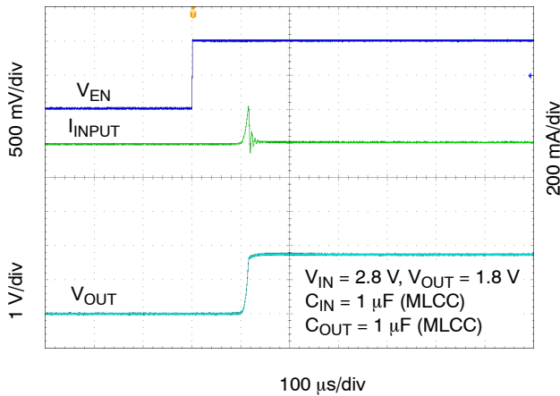
Figure 38. Enable Turn-on Response – C_{OUT} = 1\text{ μF} , I_{OUT} = 10\text{ mA}
