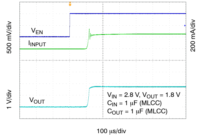
Figure 39. Enable Turn-on Response – C_{OUT} = 1\text{ μF} , I_{OUT} = 250\text{ mA}
