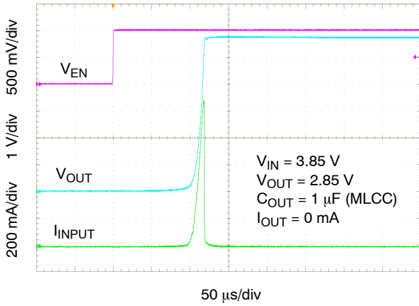
Figure 36. Enable Turn-on Response – C OUT = 1 μF – “A” Option – Normal
