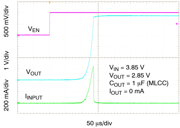
Figure 37. Enable Turn-on Response – C OUT = 1 μF – “C” Option – Slow
