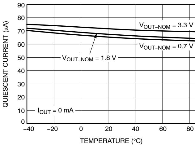
Figure 13. Quiescent Current vs. Temperature
