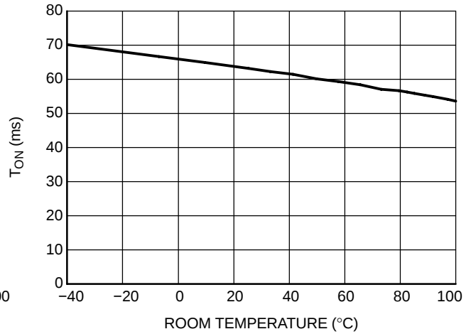
Figure 17. Turn On Time versus Room Temperature @ V_{BAT} = 3.6 V, C_{BYF} = 1 \mu F , C_{IN} = 100 nF, R_{IN} = 22 k, R_F = 110 k
