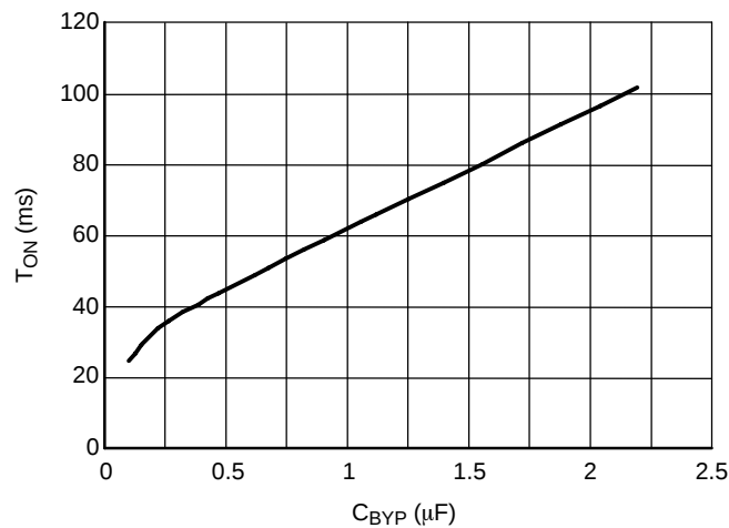
Figure 18. Turn On Time versus C_{BYF} @ V_{BAT} = 3.6 V, T_A = +25^\circ C , C_{IN} = 100 nF, R_{IN} = 22 k, R_F = 110 k
