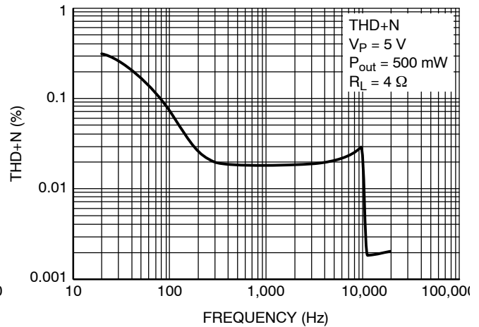
Figure 8. THD+N vs. Frequency, Single-Ended Input
