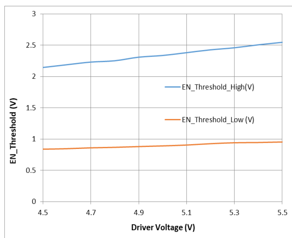
Figure 21. EN Threshold vs. Driver Voltage
