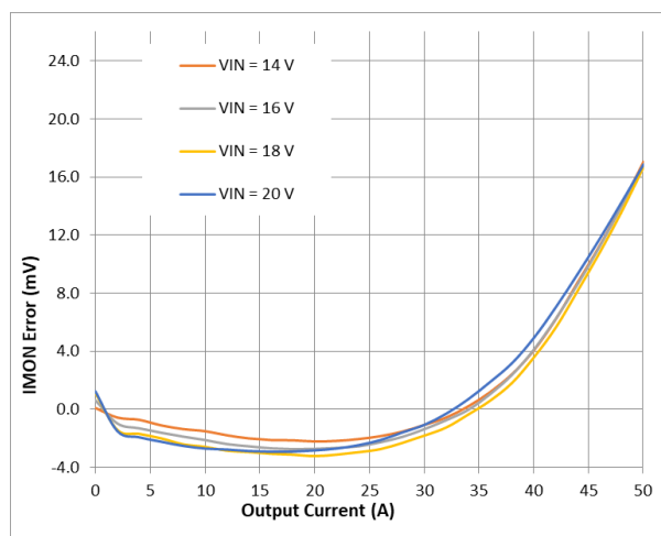
Figure 25. I_{MON} Accuracy vs. Input Voltage
