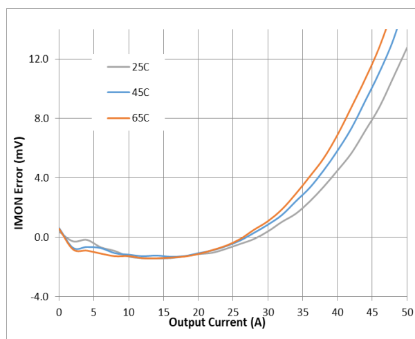
Figure 23. I_{MON} Accuracy vs. Temperature
