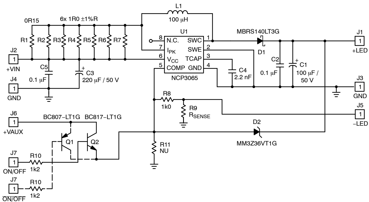
Figure 22. Boost Demo Board Application Schematic
