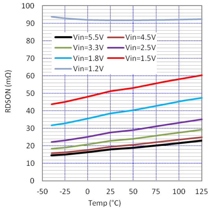
Figure 7. R DS(on) (mΩ) versus Temperature (I LOAD = 100 mA)
