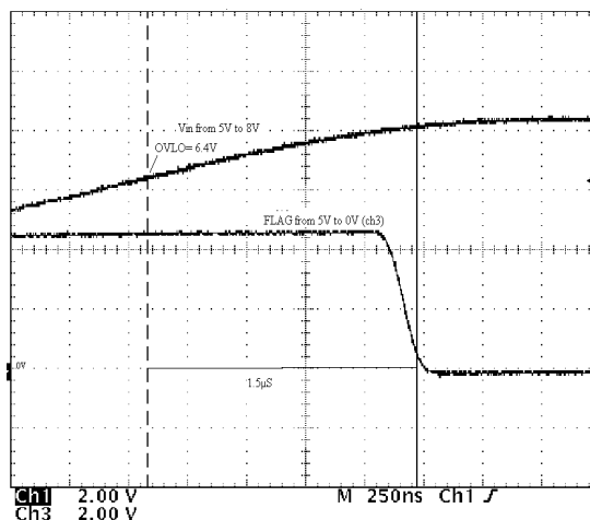
Figure 10. Alert Delay V_{out} = \text{Ch1}, \text{FLAG} = \text{Ch3}
