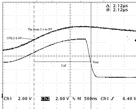
Figure 8. Output Turn Off Time V_{in} = \text{Ch1}, V_{out} = \text{Ch2}
