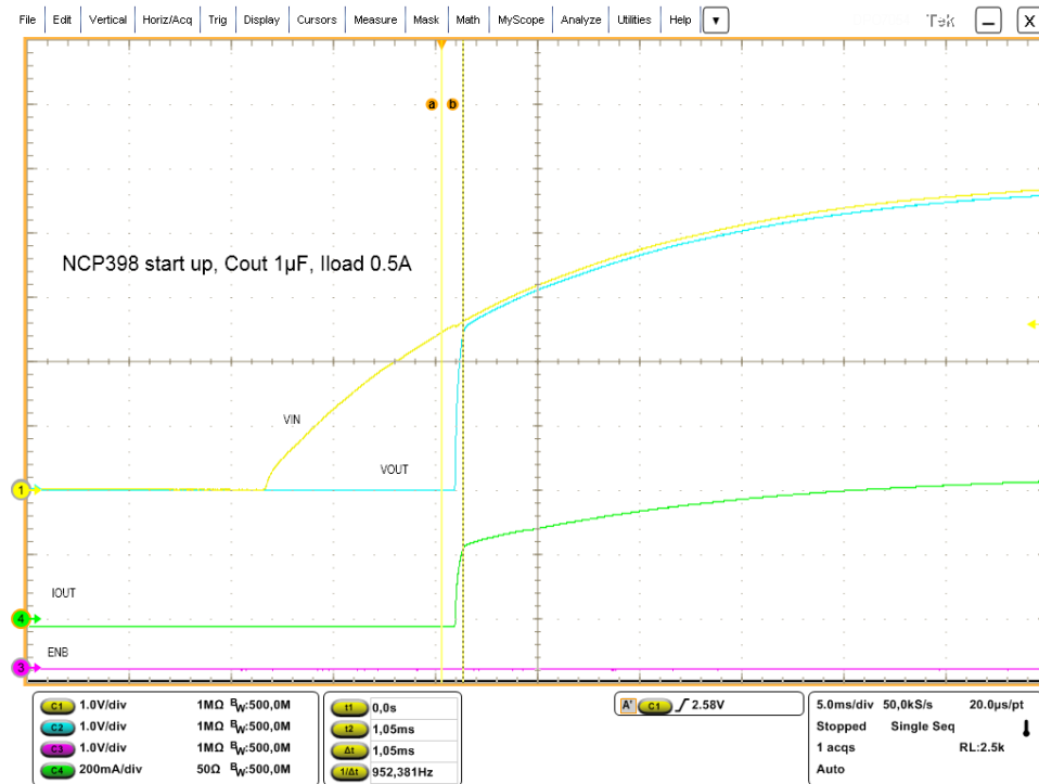
Figure 10. Soft Start Up On Load, Vin: yellow, Vout: blue, \overline{EN} : pink, IOUT: green
