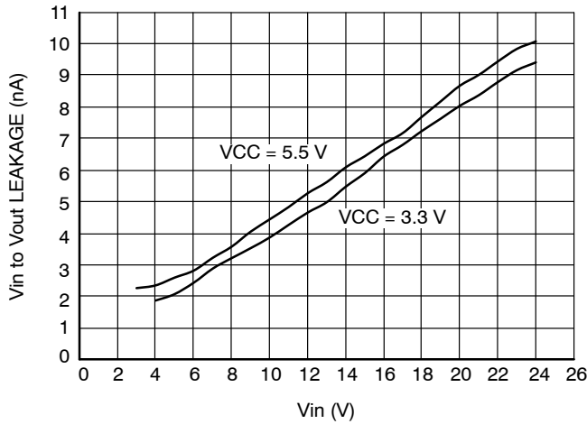
Figure 9. Input to Output Leakage vs. Input Voltage ( \text{EN} = 0 \text{ V} )
