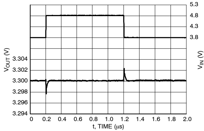
Figure 50. Line Transients, 3.3 V Version, t_R = t_F = 5 \mu s, I_{OUT} = 30 mA, AE = V_{IN} V
