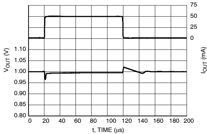
Figure 52. Load Transients, 1.0 V Version, I_{OUT} = 1 - 50 mA, t_R = t_F = 0.5 \mu s, V_{IN} = 2.0 V, AE = V_{IN} V
