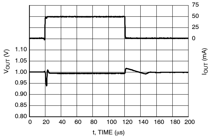
Figure 51. Load Transients, 1.0 V Version, I_{OUT} = 1 - 50 mA, t_R = t_F = 0.5 \mu s, V_{IN} = 2.0 V, AE = 0 V
