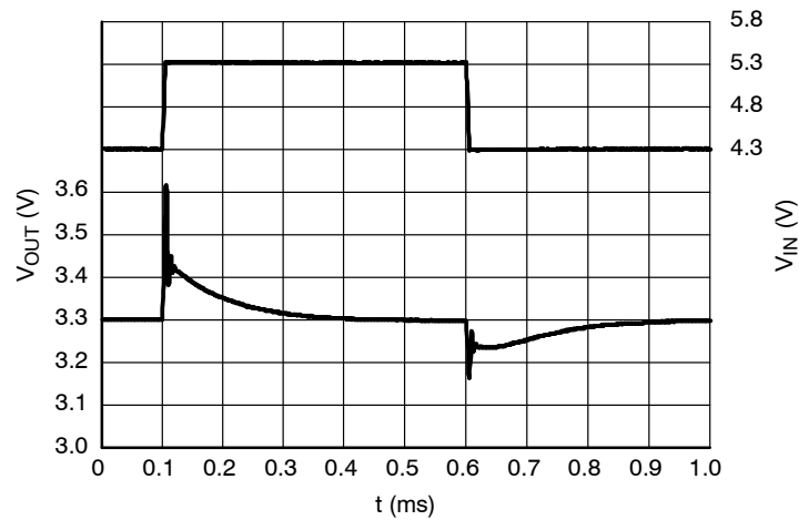
Figure 25. Line Transients, 3.3 V Version, t_R = t_F = 5 \mu s , I_{OUT} = 30 mA
