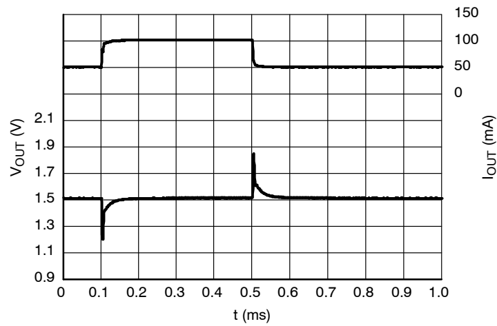
Figure 26. Load Transients, 1.5 V Version, I_{OUT} = 50 - 100 mA, t_R = t_F = 0.5 \mu s , V_{IN} = 2.5 V
