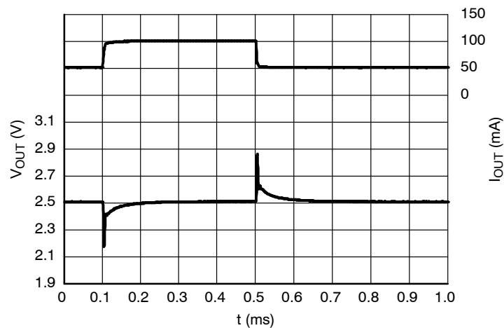
Figure 27. Load Transients, 2.5 V Version, I_{OUT} = 50 - 100 mA, t_R = t_F = 0.5 \mu s , V_{IN} = 3.5 V
