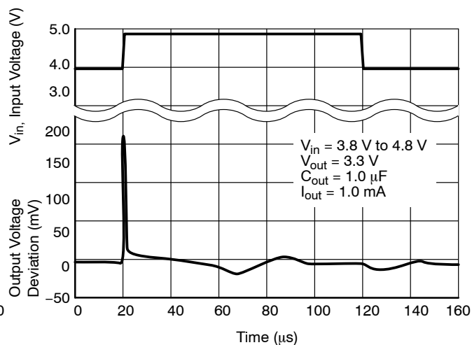
Figure 19. Line Transient Response
