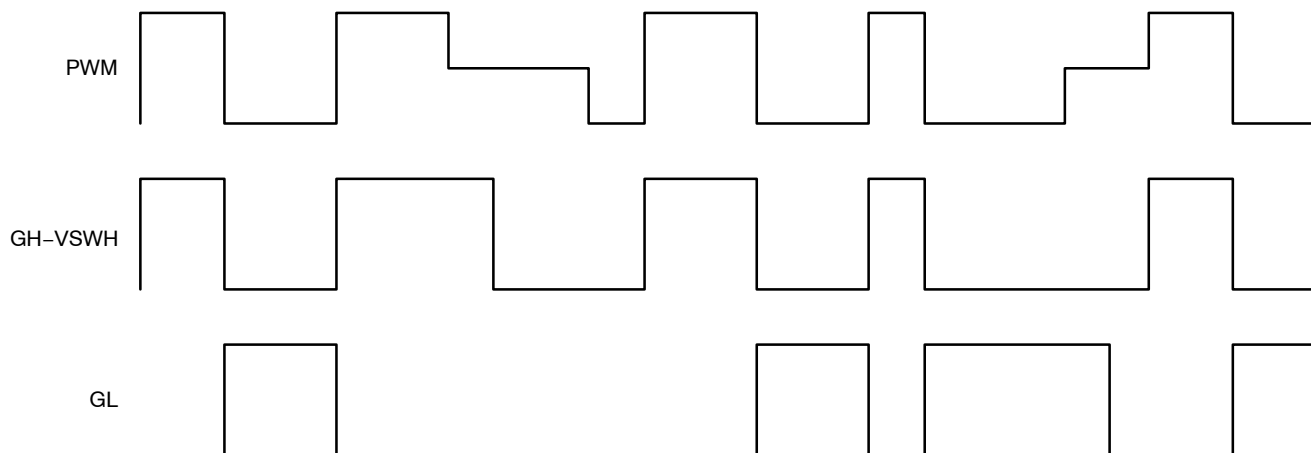
Figure 4. Timing Diagram
