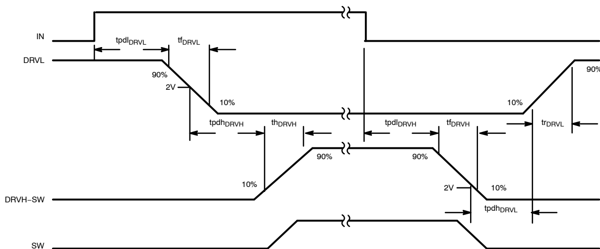
Figure 2. Timing Diagram
