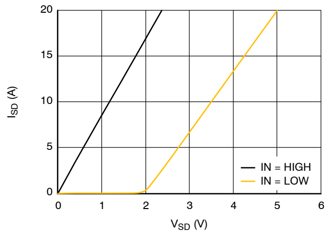
Figure 10. Typical VSD Drop vs. I DS and I N = 0 V at T J = 150°C
