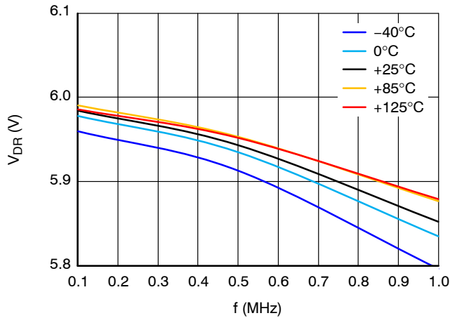
Figure 19. V_{DR} Driver Voltage vs. Frequency, R_{ON} = 0 \Omega
