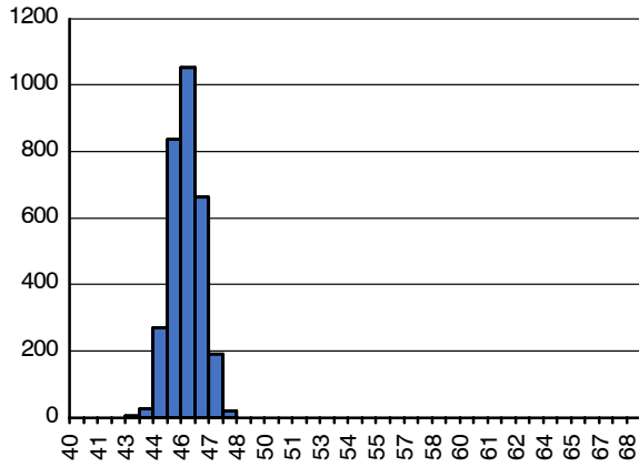
Figure 7. R DS(on) Histogram
