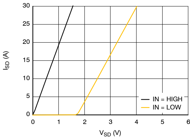
Figure 9. Typical VSD Drop vs. I DS and I N = 0 V at T J = 25°C
