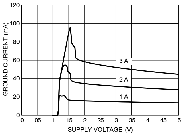
Figure 10. Ground Current vs. Supply Voltage (1.24 V)
