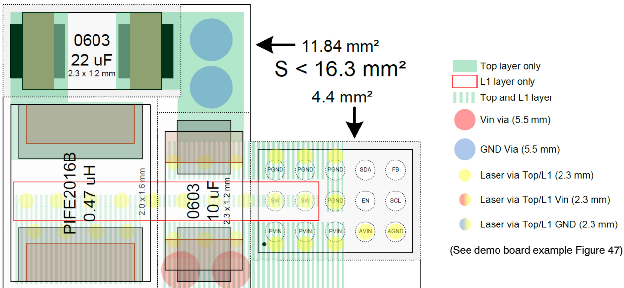
Figure 46. Layout Recommendation
