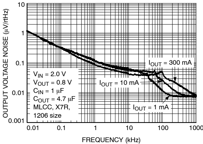
Figure 4. Output Voltage Noise Spectral Density for V_{\text{OUT}} = 0.8 \text{ V} , C_{\text{OUT}} = 4.7 \mu\text{F}
