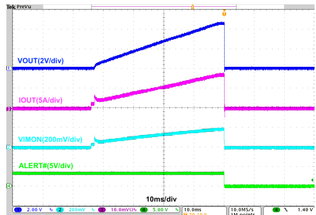
Figure 28. Over Current Protection During Softstart
