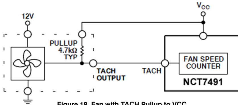
Figure 18. Fan with TACH Pullup to VCC
