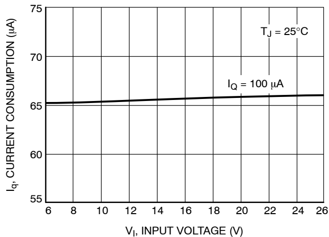
Figure 25. Current Consumption vs. Input Voltage
