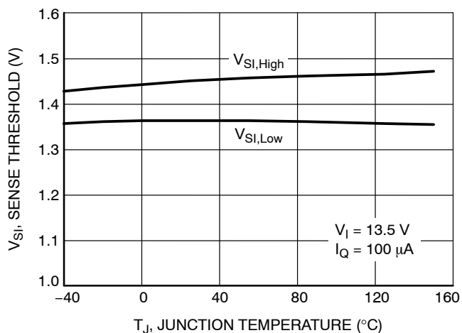
Figure 27. Sense Threshold vs. Junction Temperature
