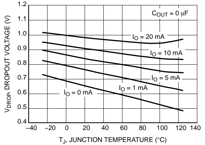
Figure 5. Dropout Voltage
