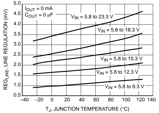
Figure 7. Line Regulation
