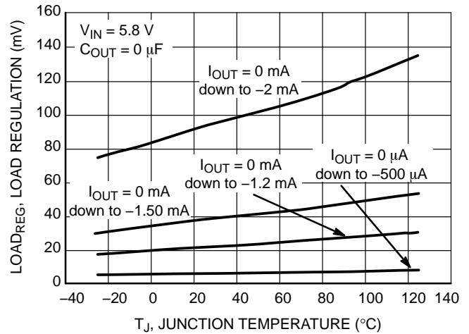
Figure 9. Load Regulation Sinking
