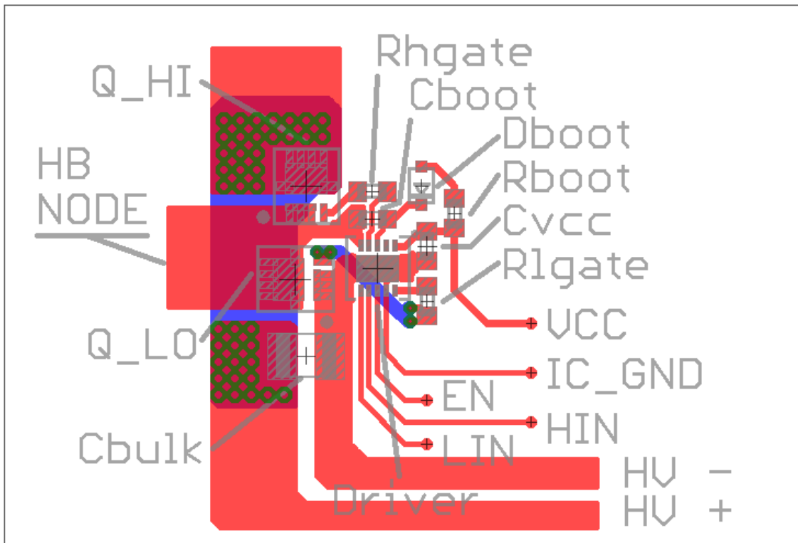
Figure 51. Recommended Layout
