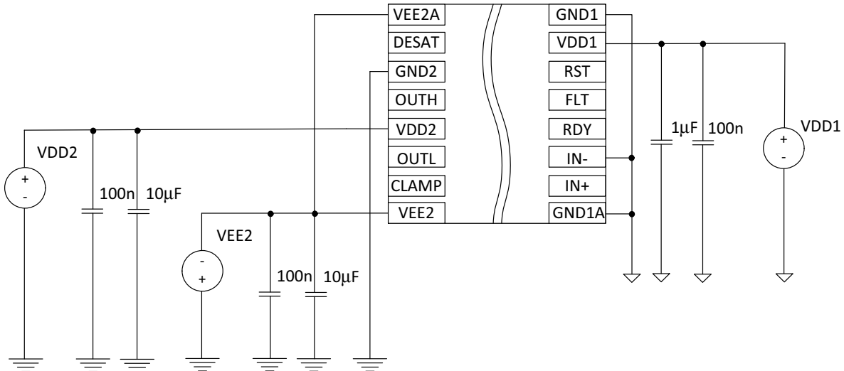
Figure 24. Bipolar Power Supply
