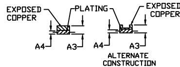
DETAIL B
