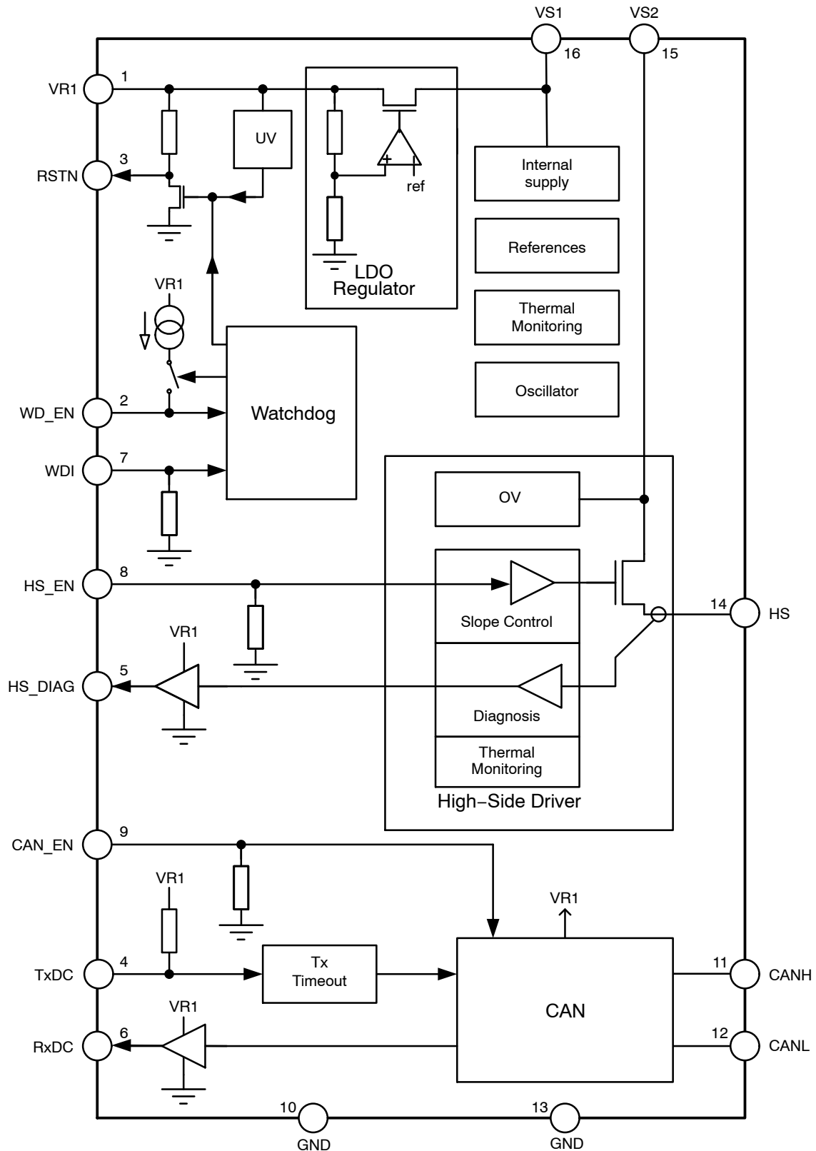
Figure 2. Block Diagram
