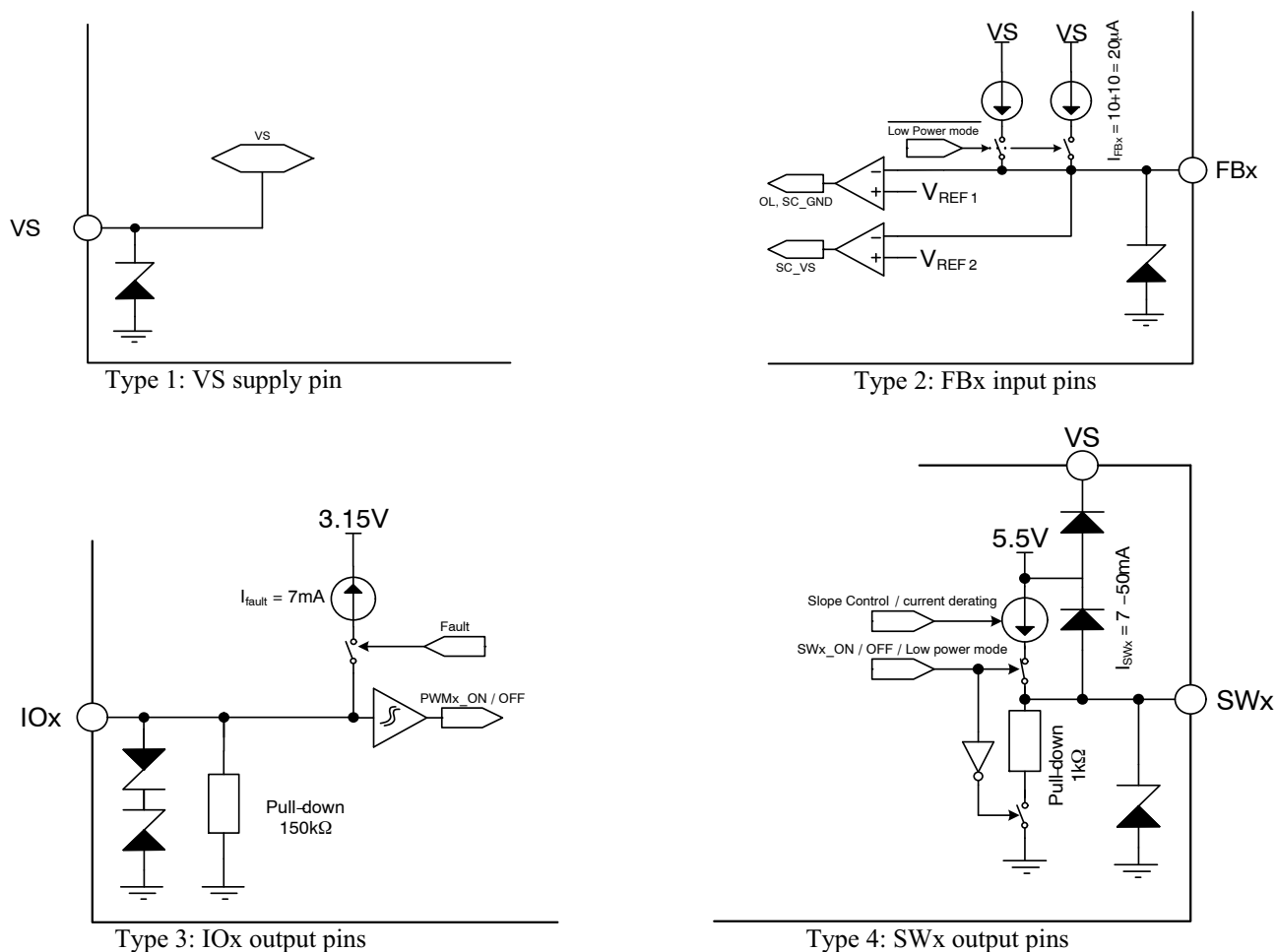
Figure 3. Input and Output Equivalent Diagrams
