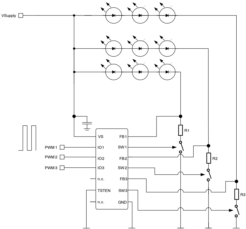
Figure 1. Application Diagram
