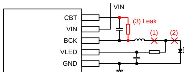
Figure 25. CBT_UV Protection
