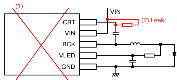
Figure 26. CBT_OV Failure
