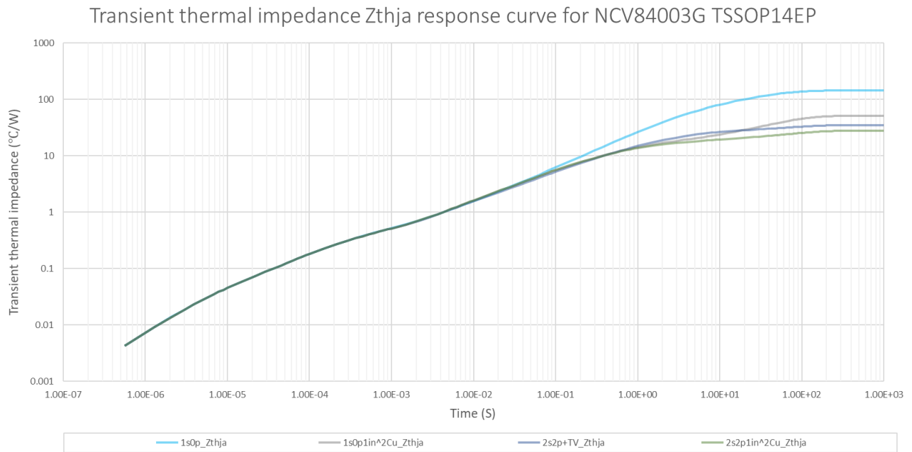
Figure 55. Transient Thermal Response
