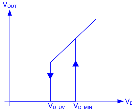
Figure 17. Under-voltage Behavior
