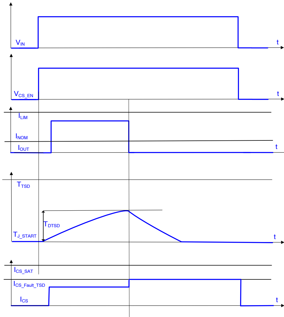
Figure 27. Over-Temperature Protection
