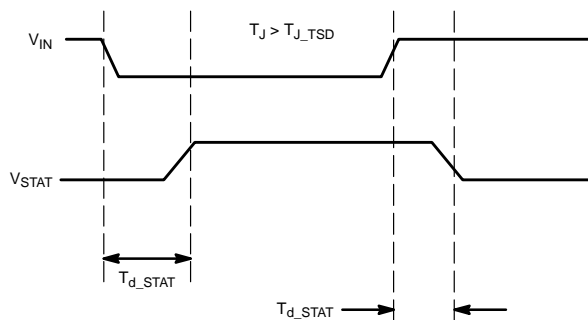
Figure 3. Overtemperature Status Timing
