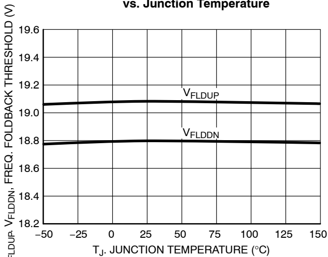
Figure 14. Rising Frequency Foldback Threshold vs. Junction Temperature
