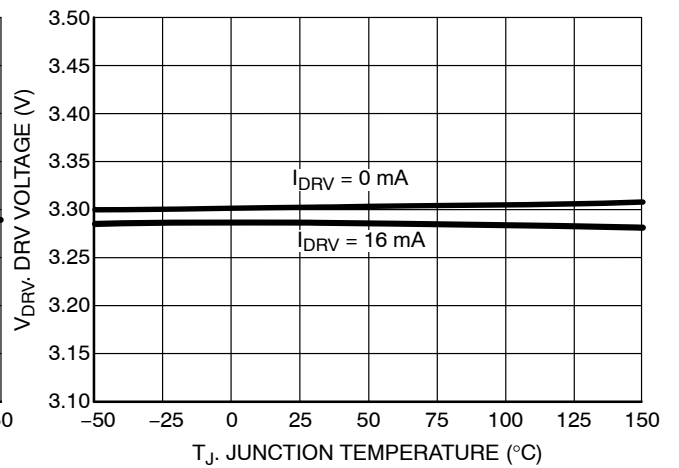
Figure 21. DRV Voltage vs. Junction Temperature
