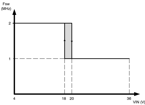
Figure 25. NCV890103 Switching Frequency Reduction at High Input Voltage
