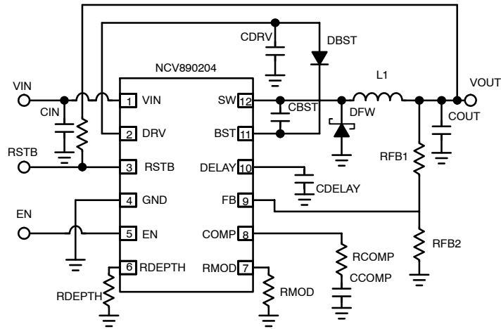
Figure 1. Typical Application
