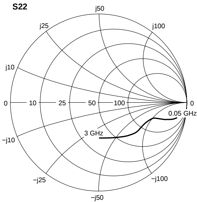
Figure 13. Output Reflection Coefficient
