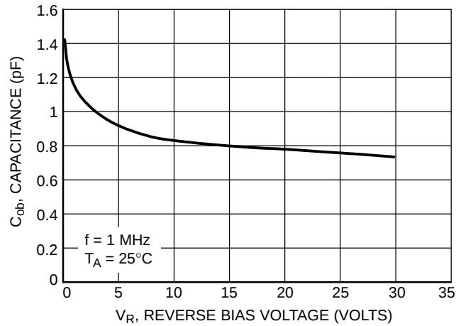
Figure 6. Output Capacitance
