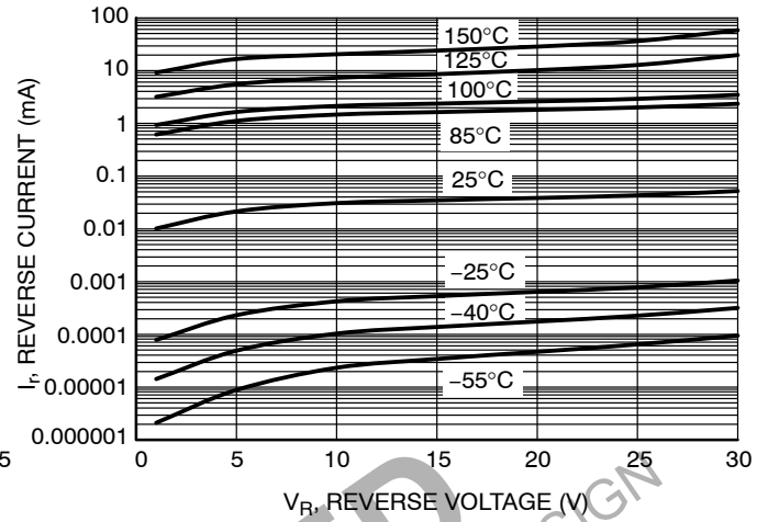
Figure 6. Leakage Current
