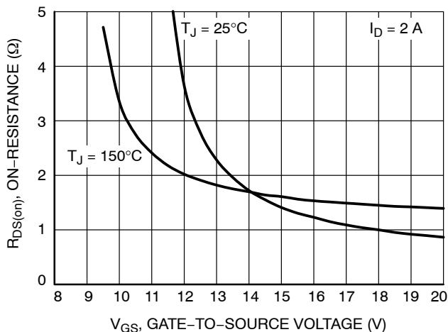
Figure 6. On-Resistance vs. Gate-to-Source Voltage
