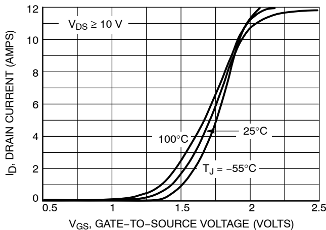
Figure 3. Transfer Characteristics
