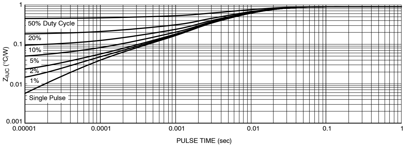
Figure 13. Thermal Impedance
