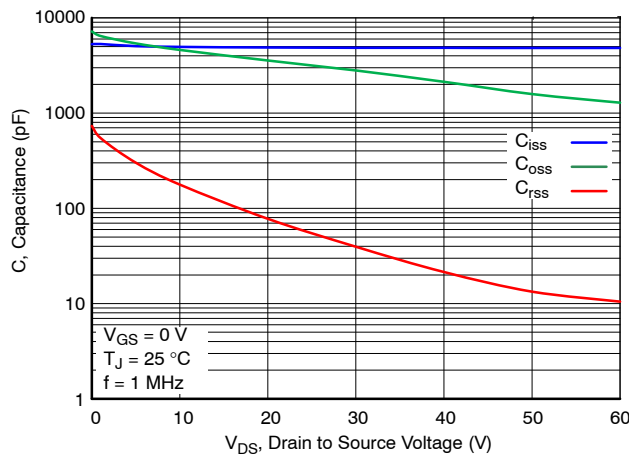
Figure 7. Capacitance Characteristics
