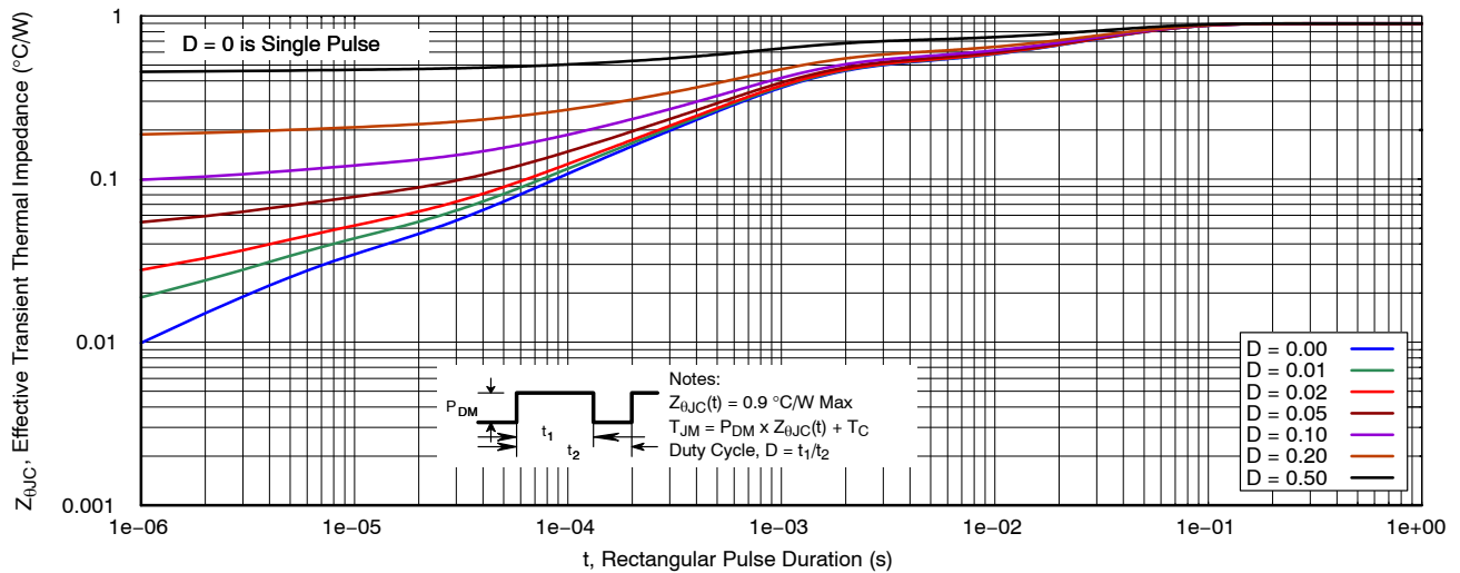
Figure 14. Transient Thermal Response
