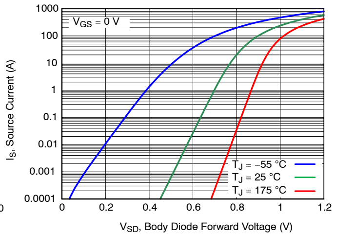
Figure 10. Diode Forward Characteristics
