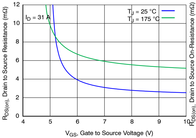
Figure 3. On-Resistance vs. Gate Voltage
