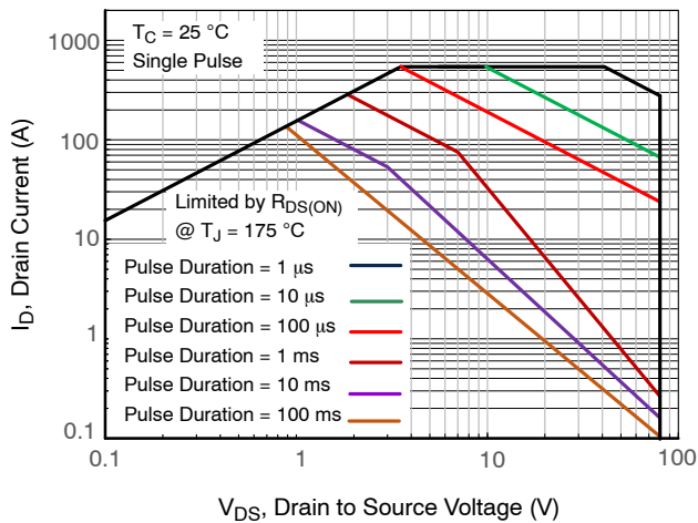
Figure 11. Safe Operating Area (SOA)
