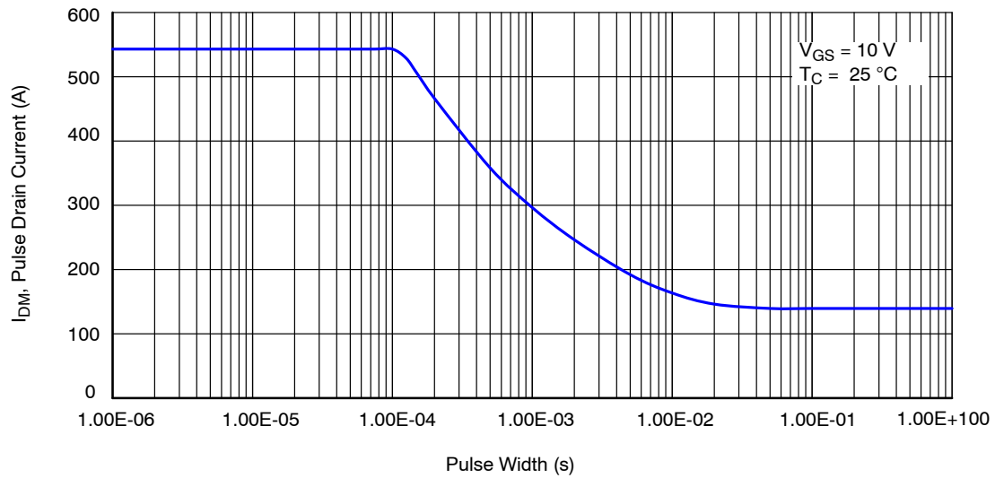
Figure 13. I_{DM} vs. Pulse
