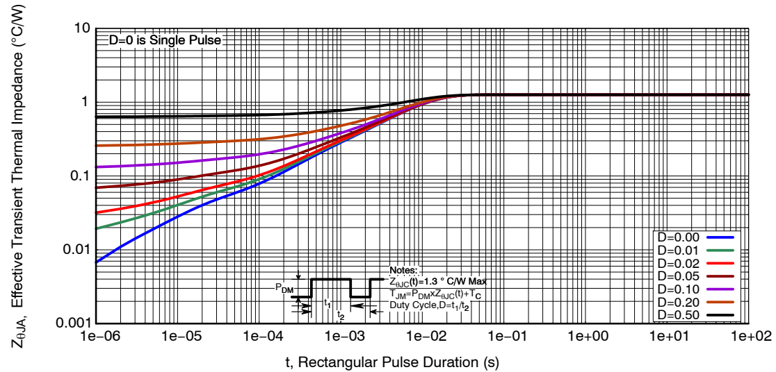
Figure 14. Transient Thermal Response
