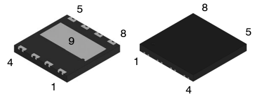
PTFP-N9 8.00x8.00x0.90, 2.00P (DFN) CASE 522AG
