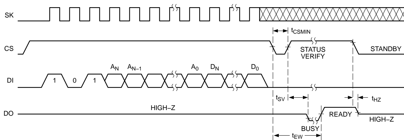
Figure 5. Write Instruction Timing
