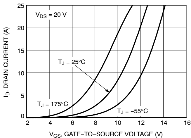
Figure 6. Transfer Characteristics
