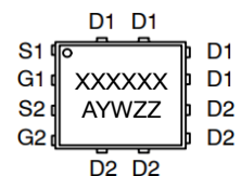
1 DFN8 5x6 (SO-8FL) CASE 506BT
