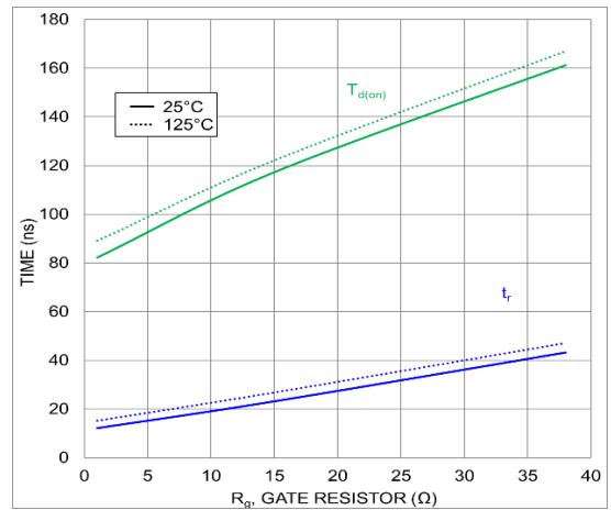
Figure 17. Typical Turn-On Switching Time vs. R_g
