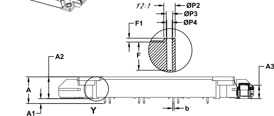
PIM11, 152.00x62.15x17.00 CASE 180HT ISSUE E
