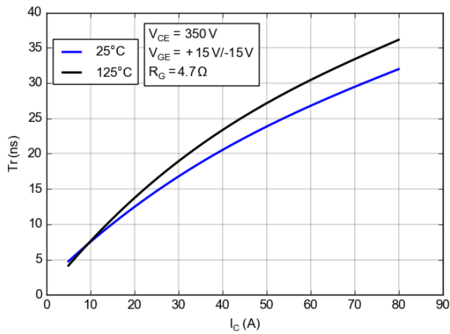
Figure 26. Typical Switching Times Tron vs. I_C
